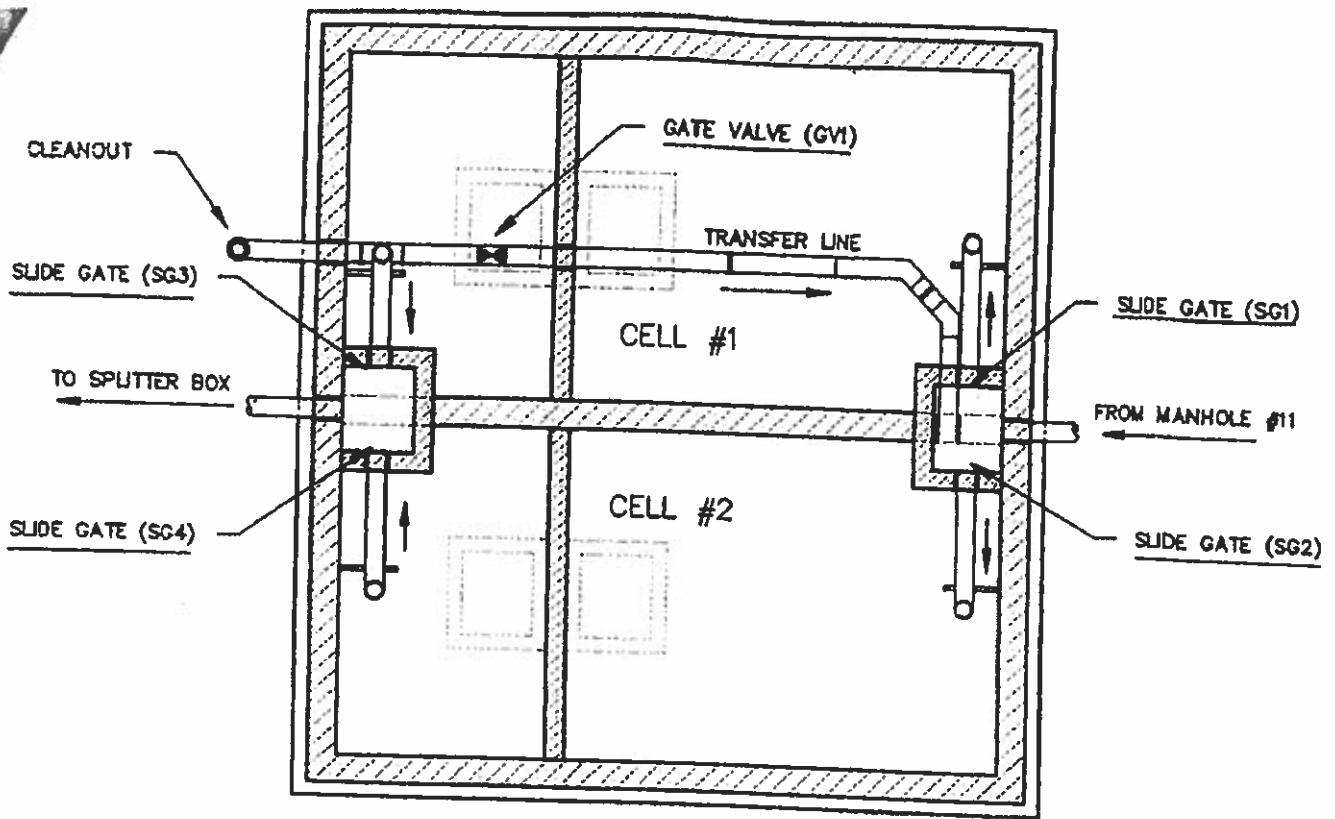
SEPTIC TANK - PLAN VIEW SCALE: NONE
