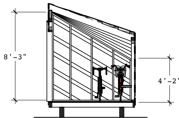
SECTION 3/16TH SCALE
