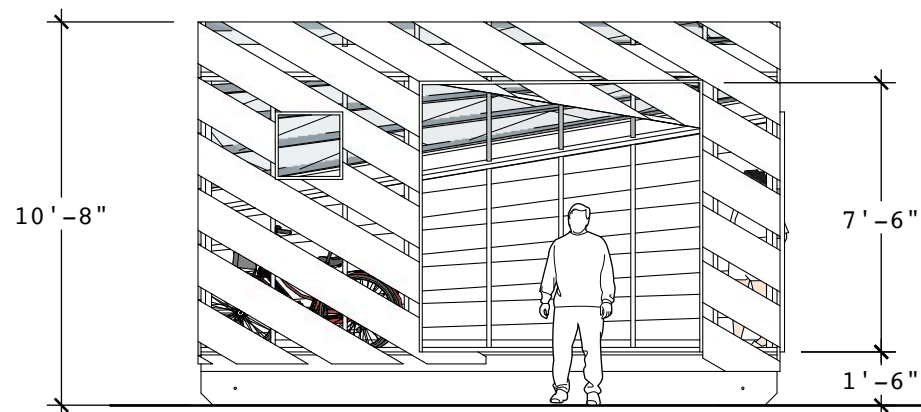
STREET SIDE ENTRY 3/16TH SCALE
