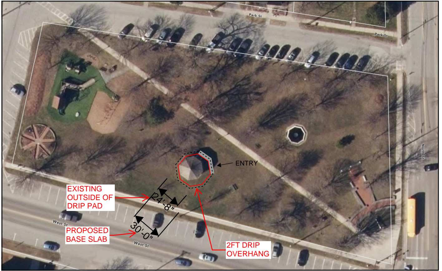
SITE PLAN
