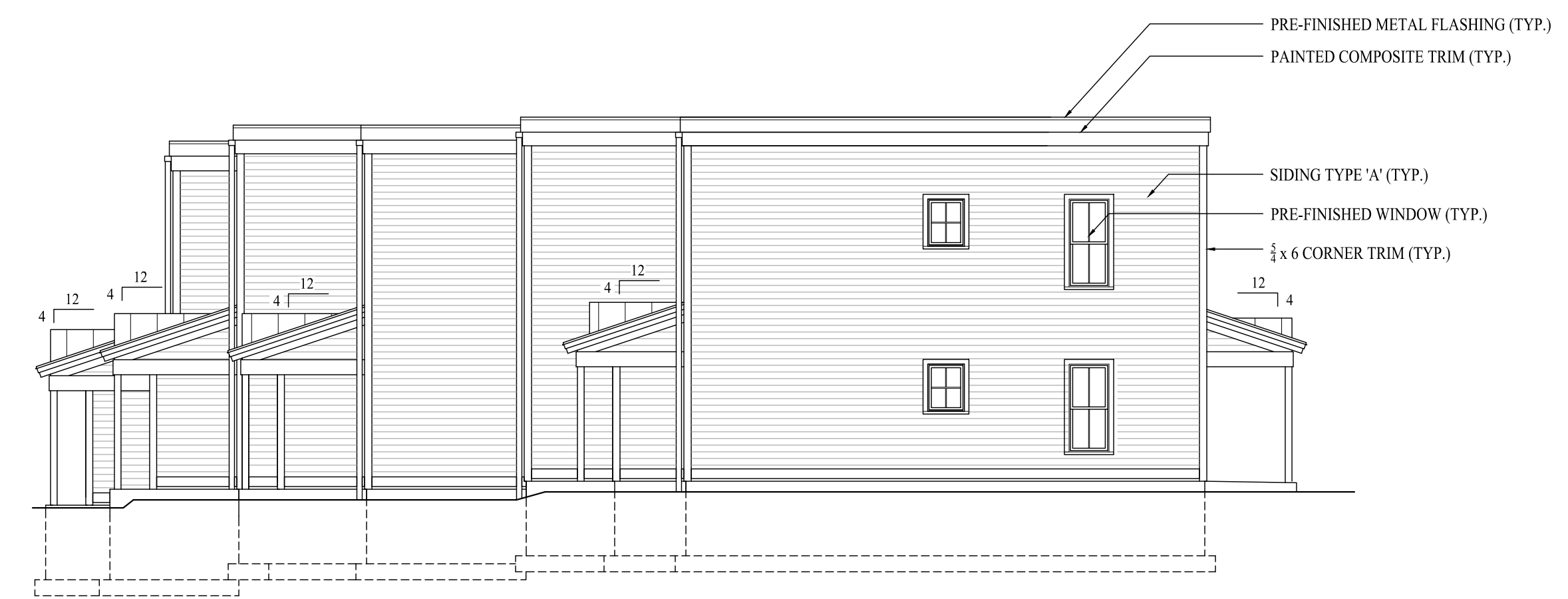
3 NORTH ELEVATION - BUILDING 'A' A-2.0 1/8" = 1'-0"
