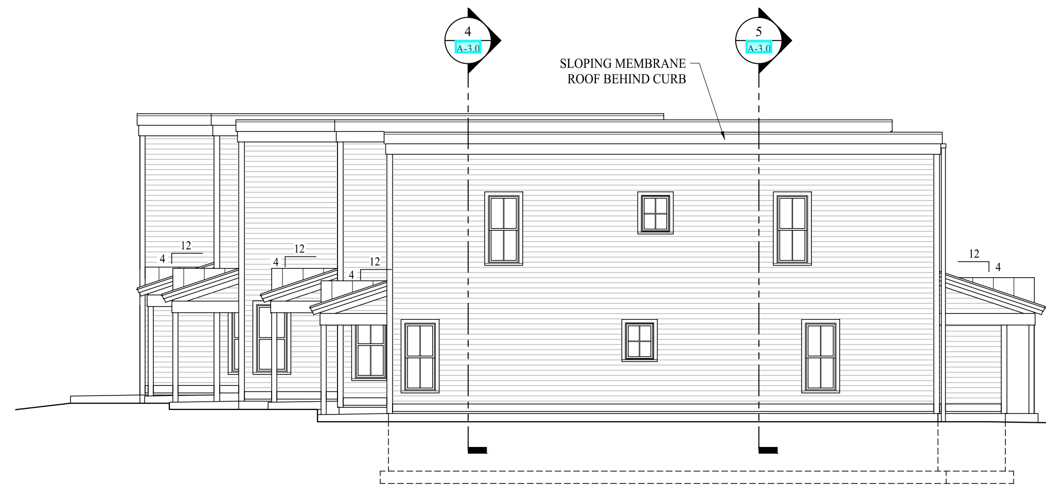
4 WEST ELEVATION - BUILDING 'A' A-2.0 1/8" = 1'-0"
